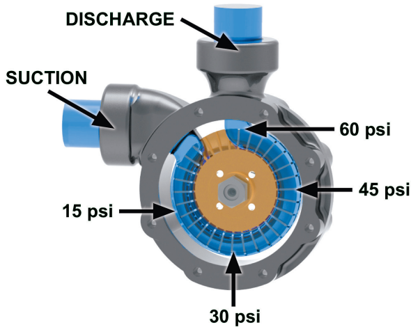
1 Pressure produced by a turbine pump increases continuously from suction to discharge
