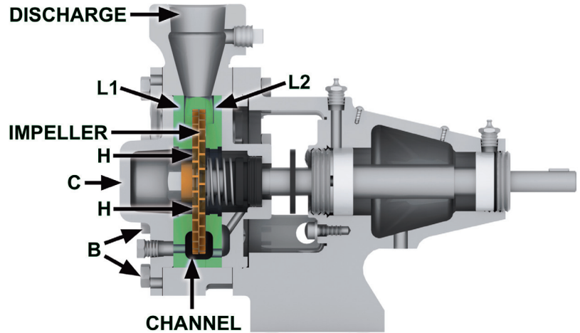
2 Cross section of a turbine pump. Vanes cut in the impeller's rim revolve in an annular channel where pressure is produced to helical rotation of the liquid
